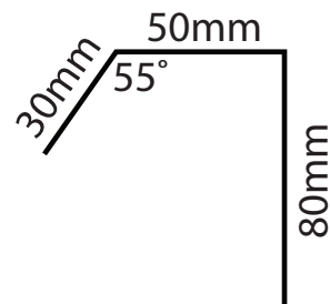
Custom Glaze Barge Capping
