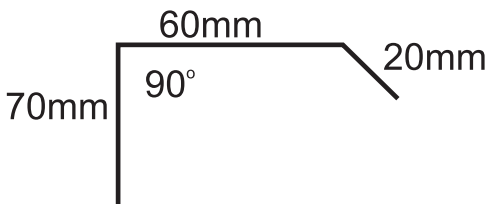
Barge Capping
