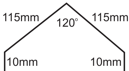
Ridge Capping
