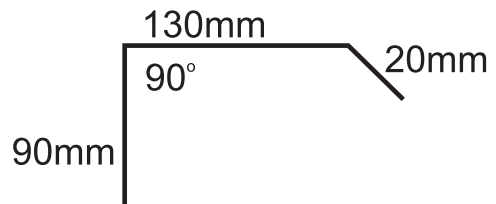
Barge Capping
