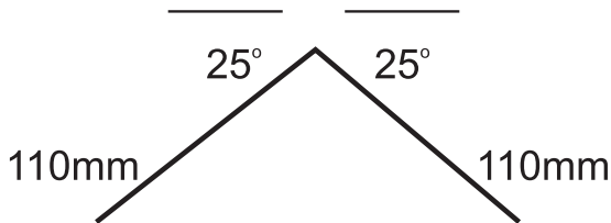
Ridge Capping
